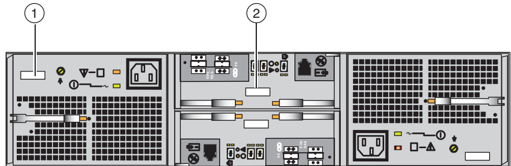
Figure 37 Example of 2U, 25 (2.5-inch) DAE LCC and power supply
