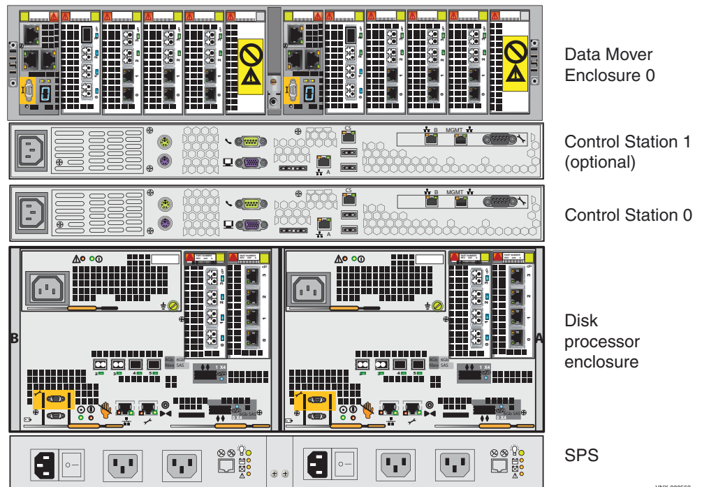
Figure 3 Example of Block and File VNX5300 platform (rear view)
