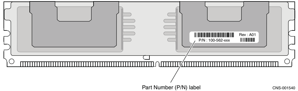
Figure 31 Example of the Block and File VNX5300 platform SP DIMM part number location
