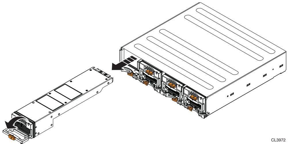
Figure 16 Example of the Data Mover power supply/cooling fan module removal
