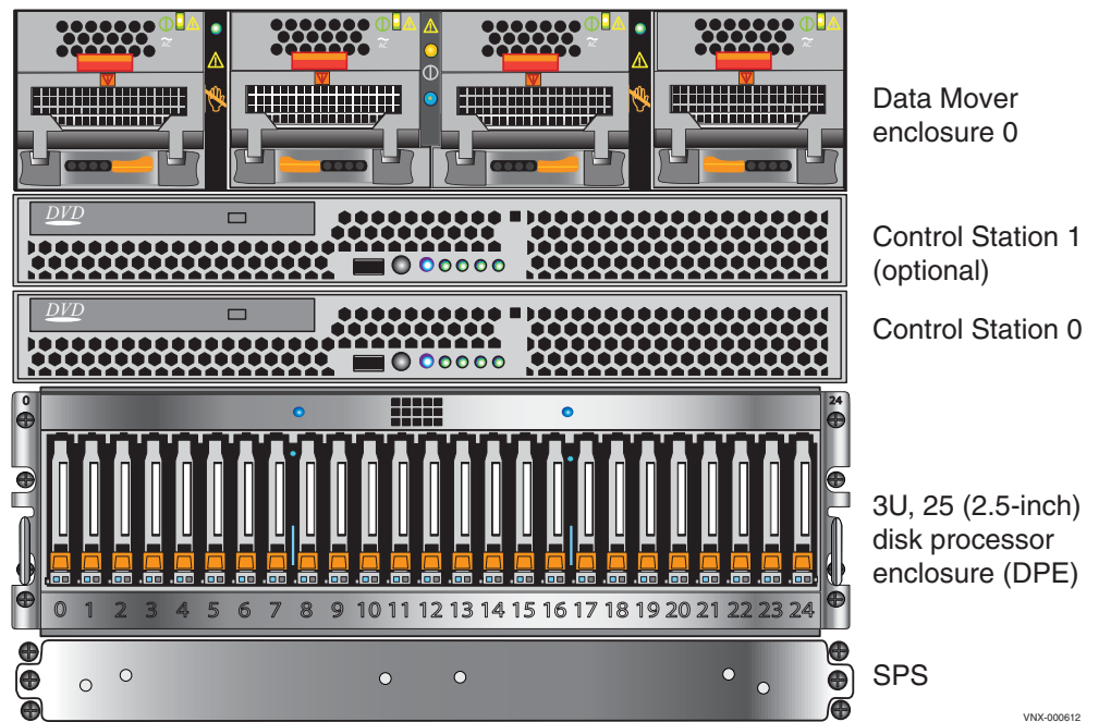
Figure 2 Example of the Block and File VNX5300 platform with a 3U, 25 (2.5-inch) DPE (front view)
