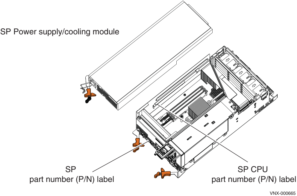
Figure 12 Example of the SP CPU with power supply/cooling module set aside
