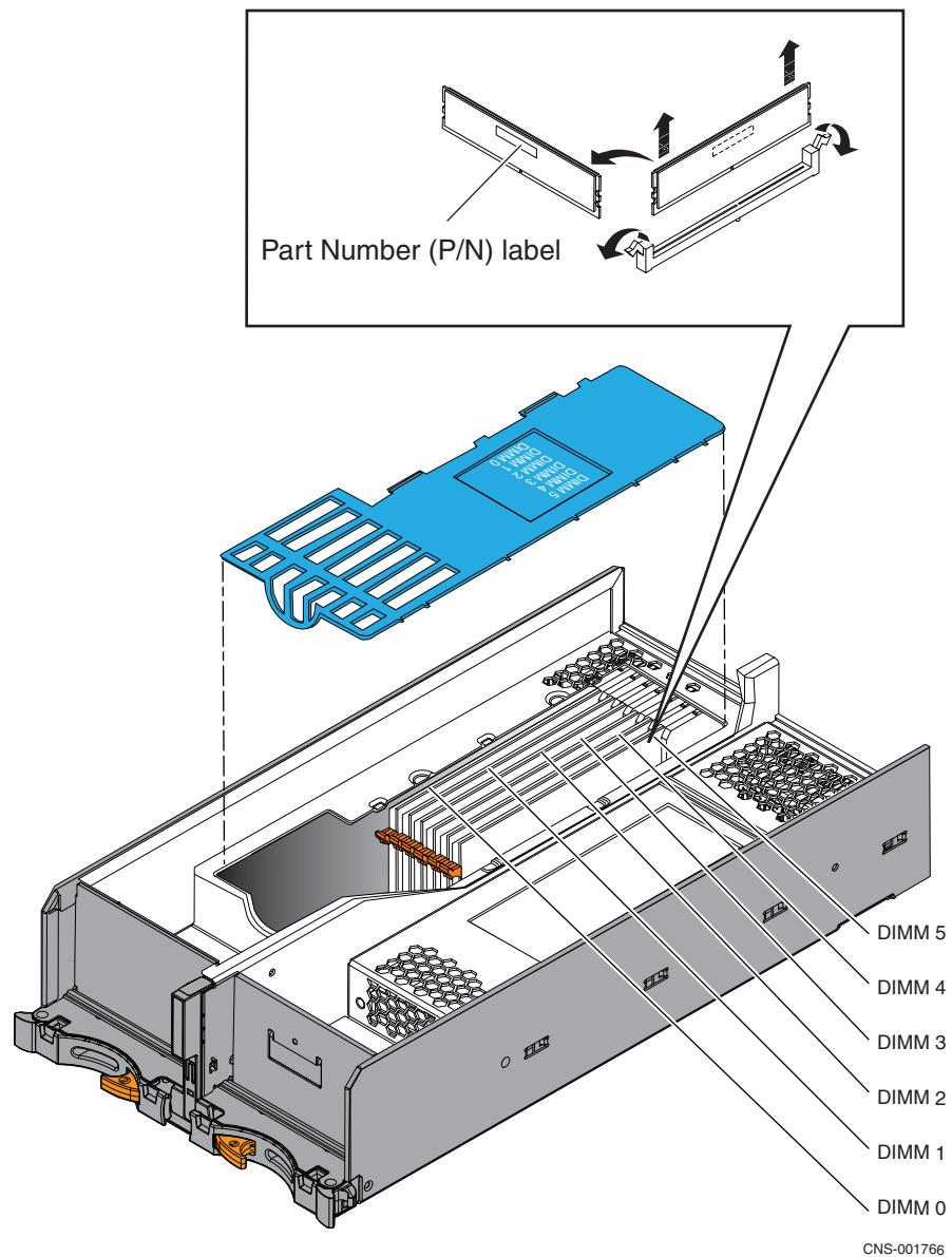
Figure 32 Example of the Block and File VNX5300 platform Data Mover DIMM slot location
