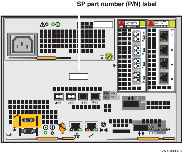
Figure 9 Example of an SP
