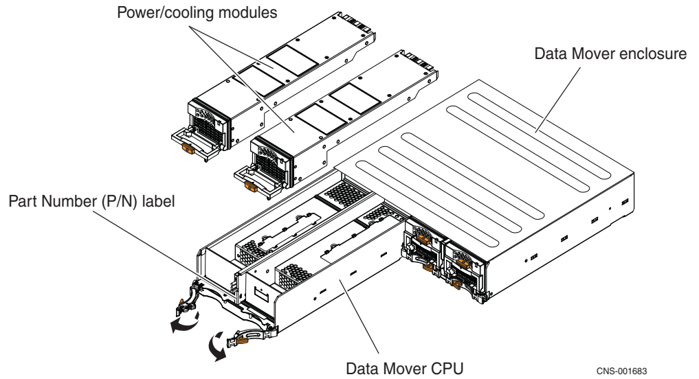
Figure 17 Example of the Data Mover CPU being removed from a Data Mover enclosure
