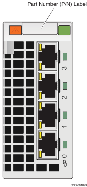
Figure 27 Example of the four-port 1-Gb/s copper I/O module
