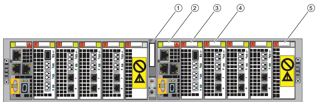
Figure 18 Data Mover enclosure (rear view)
