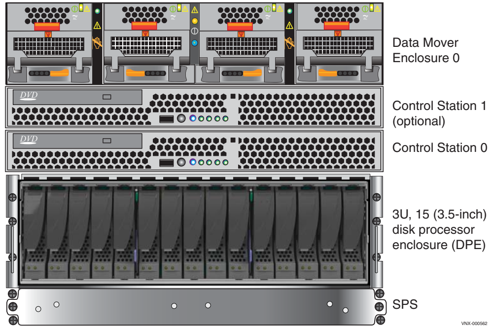
Figure 1 Example of the Block and File VNX5300 platform with a 3U, 15 (3.5-inch) DPE (front view)
