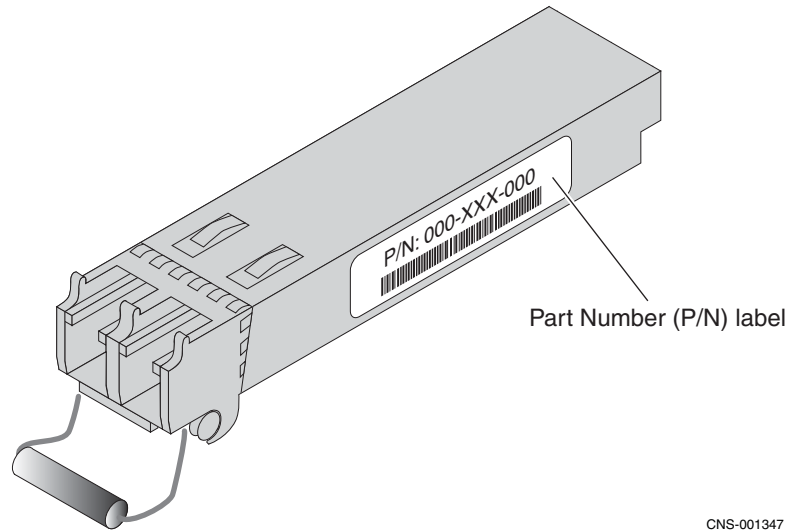
Figure 29 Example of an SFP with a bale clasp
