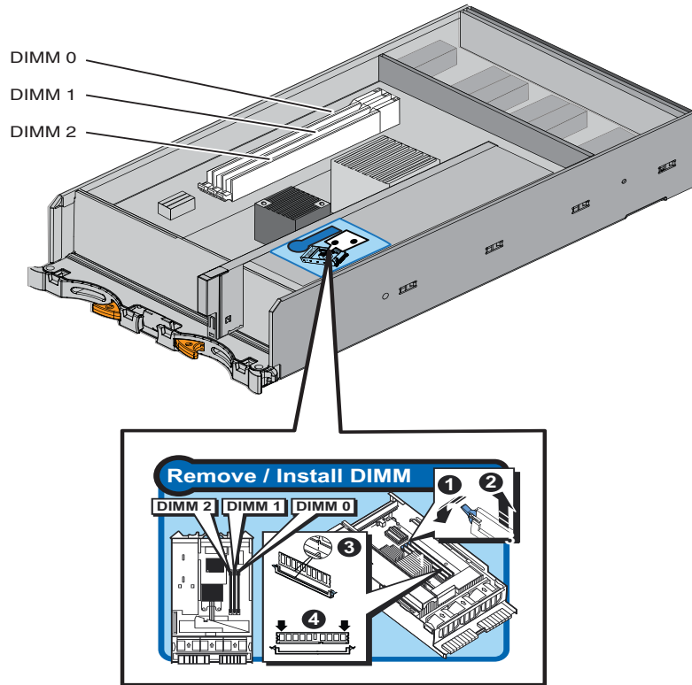
Figure 30 Example of the Block and File VNX5300 platform SP DIMM slot location
