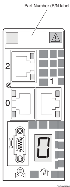
Figure 19 Example of the Data Mover enclosure management module
