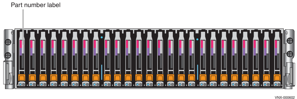
Figure 35 Example of the 2U, 25 (2.5-inch) disk drive DAE (front view)
