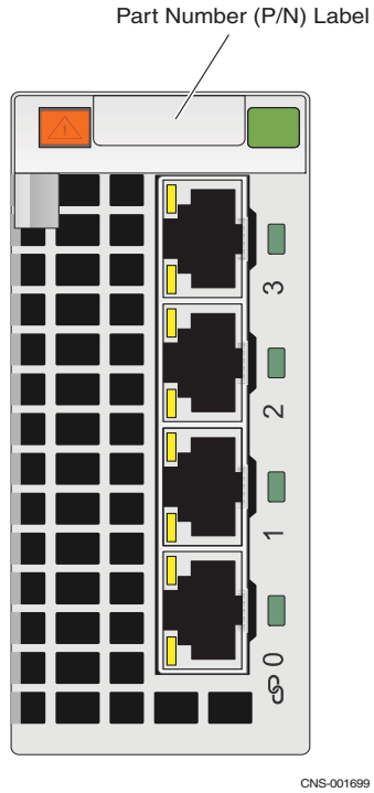
Figure 21 Example of the four-port 1-Gb/s copper iSCSI I/O module
